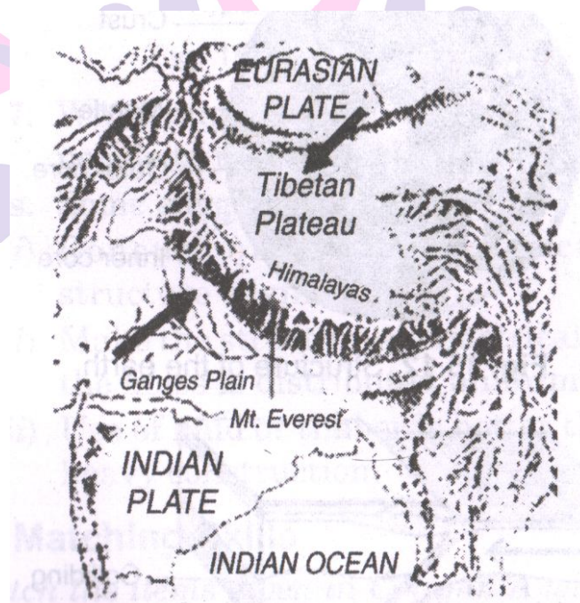
Movements of Indian earth's plate
